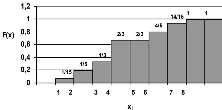
Figure 2.1 – The graphs of function F(x)
