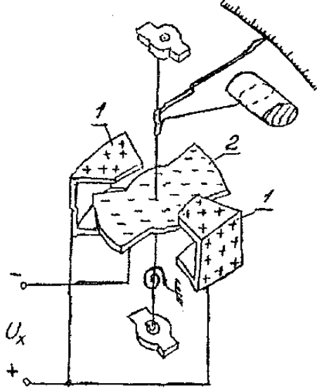
Figure 1.6 – Electrostatic mechanism.
