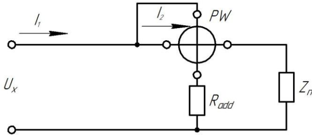
Figure 1.5 – Wattmeter's scheme.
