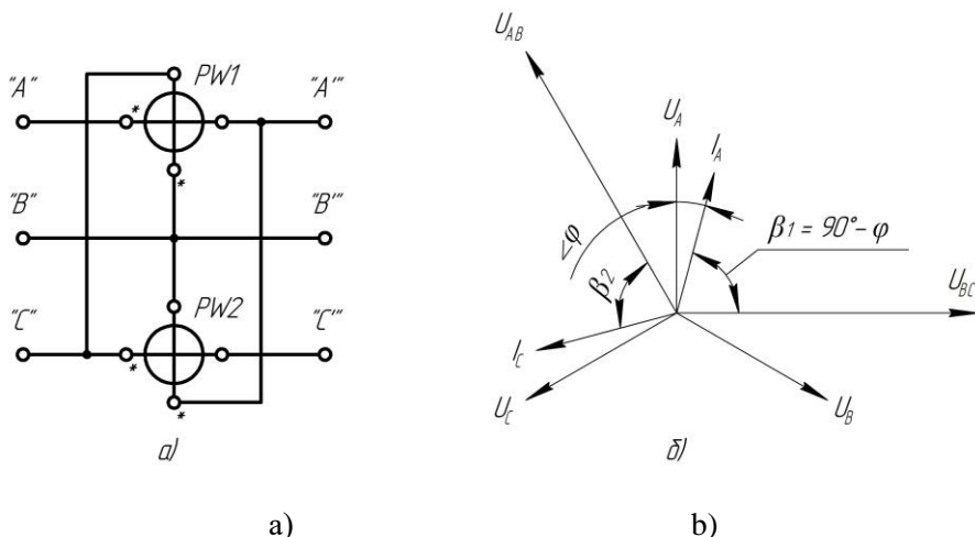
Figure 3.5 – Circuit Diagram (a) and Vector Diagram (b) for Measuring Reactive Power Using the Two-Instrument Method.
