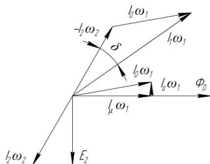
Figure 4.2 – Vector Diagram of the Current Transformer.
