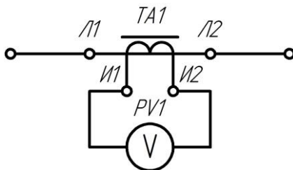
Figure 4.4 – Connection Diagram of a Voltmeter in the Secondary Circuit of a Current Transformer.
