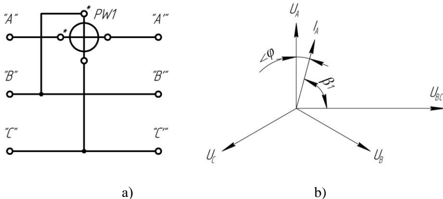
Figure 3.4 – Circuit Diagram (a) and Vector Diagram (b) for Measuring Reactive Power Using the Single-Instrument Method.
