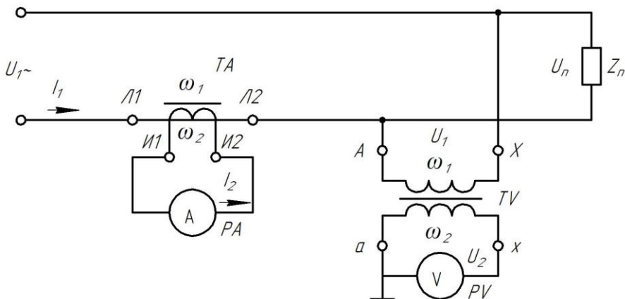
Figure 4.1 – Connection Diagram of Current and Voltage Transformers.
