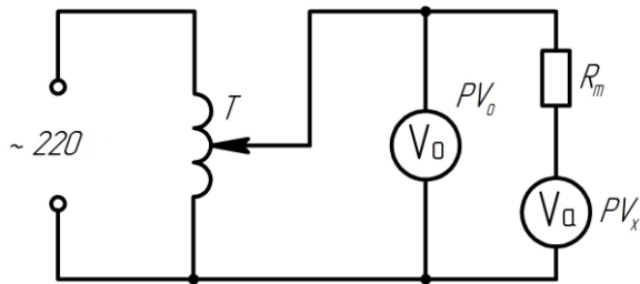
Figure 2.3 – Laboratory work scheme.
