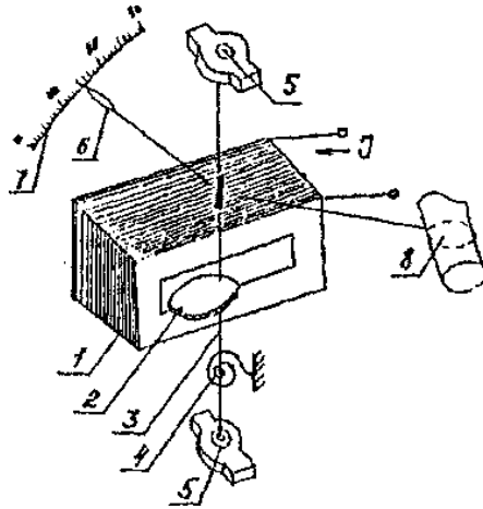
Figure 1.2 – Electromagnetic mechanism.
