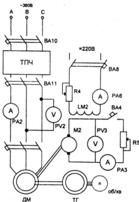
Figure 4.2 – Induction motor under frequency control by the law U / \sqrt{f} = \text{const.}
