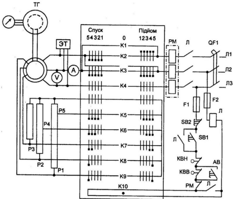
Figure 3.1 - Electric drive of the mechanism of lifting of the crane. The electric basic circuit.
