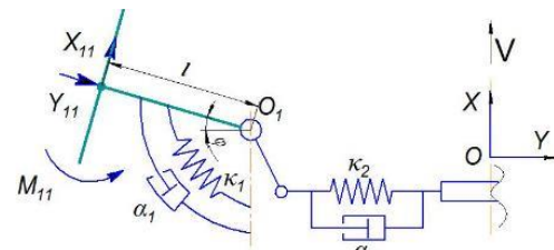
Figure 6. Schematic diagram of wheel assembly with toe-in angle
