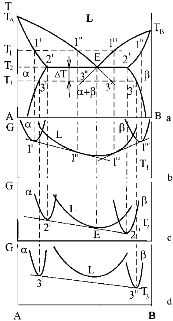
Fig. 1. Eutectic phase equilibrium diagram (a) and Gibbs free energies (b-d)
