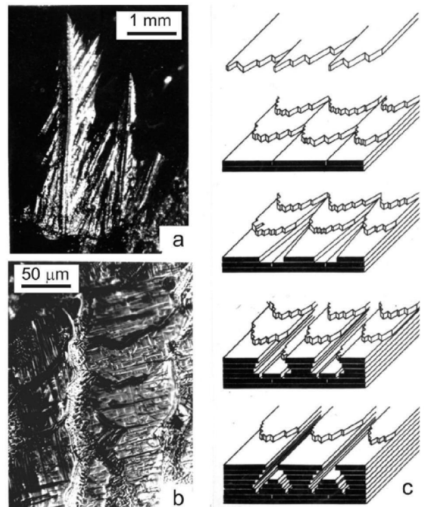
Fig. 3. Relief of primary \text{Fe}_3\text{C} crystal (a, b) after decantation in eutectic alloy Fe-4.6 % (wt.) C and its formation scheme (c)
