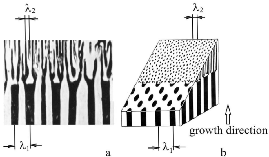
Fig. 18. The branching of rods of \gamma -Fe (dark) in moment of quenching of semi-solid ( \gamma -Fe) + \text{Fe}_3\text{C} eutectic alloy in water
