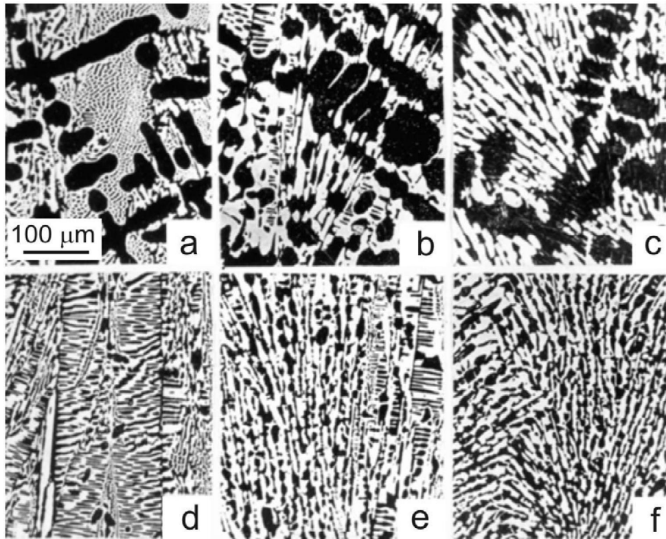
Fig. 20. Influence of a melt undercooling \Delta T on a degree of cooperativity of (\gamma\text{-Fe}) + \text{Fe}_3\text{C} eutectics in hypoeutectic (a-c) and hypereutectic (d-f) alloys: a, d – \Delta T = 5^\circ\text{C} ; b, e – \Delta T = 25^\circ\text{C} ; c, f – \Delta T = 35^\circ\text{C}
