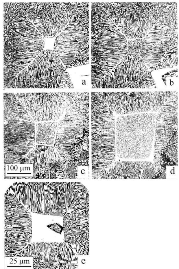
Fig. 9. The consecutive sections of Bi-Sn eutectics: a – the basic primary Bi crystal is located in center of eutectic grain; b-d – sections through five eutectic pyramids; e – growth of Sn dendrite on the plane of Bi crystal
