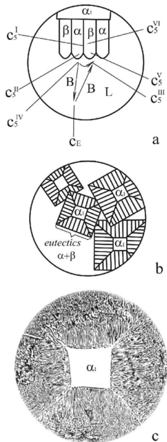
Fig. 2. Diffusion flows in liquid phase during eutectic solidification (a) and eutectic grain formation, b-morphological scheme, c- microstructure. Primary basic crystal is identified as \alpha_1
