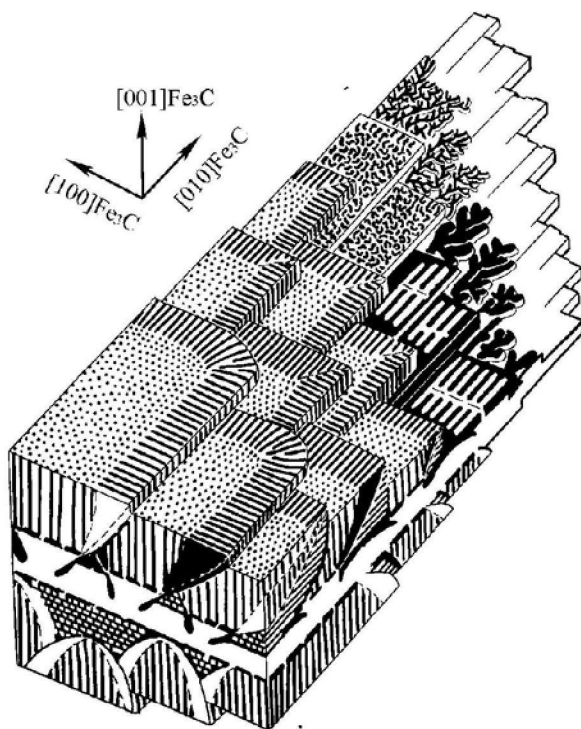
Fig. 8. 3D model of ( \gamma\text{-Fe} + \text{Fe}_3\text{C} ) eutectic
