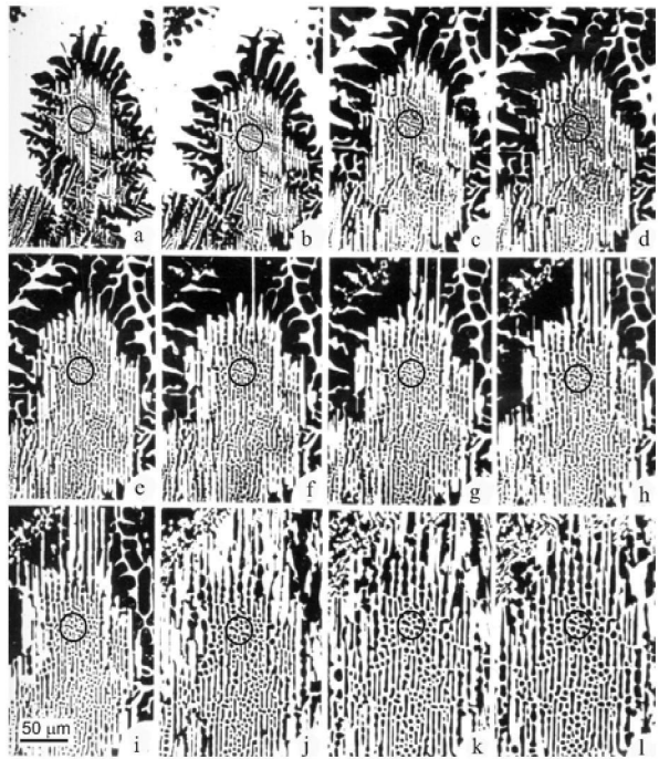
Fig. 6. Consecutive (001) \text{Fe}_3\text{C} sections of the eutectic cell. Rounded area shows a continuity of both dark austenite \gamma\text{-Fe} and white cementite \text{Fe}_3\text{C} phases
