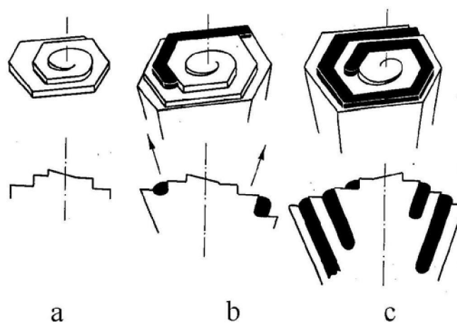
Fig. 17. The model of biphasic growth on the screw dislocation [2]: a – dislocation hill on the vertex of dendrite branch of primary \text{MgZn}_2 crystal; b – the dislocation decorated by second eutectic Zn phase (dark); c – coupled growth of eutectic phases
