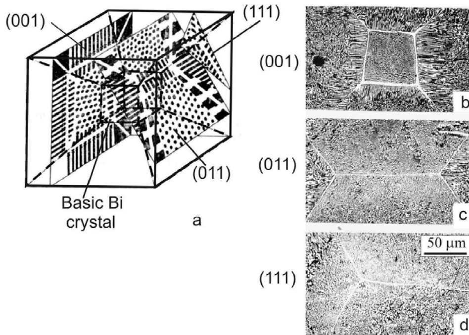
Fig. 11. Three types of inter-pyramidal boundaries in cubic eutectics Bi-Sn
