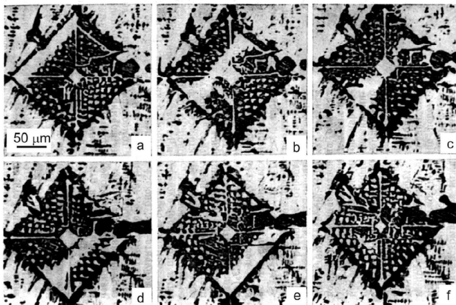
Fig. 12. Consecutive sections of the octahedral eutectic colony in Fe-Mo-C system: dark phase is \gamma -Fe and white phase is (Mo, Fe)C. The basic carbide crystal is genetic centre of eutectic colony
