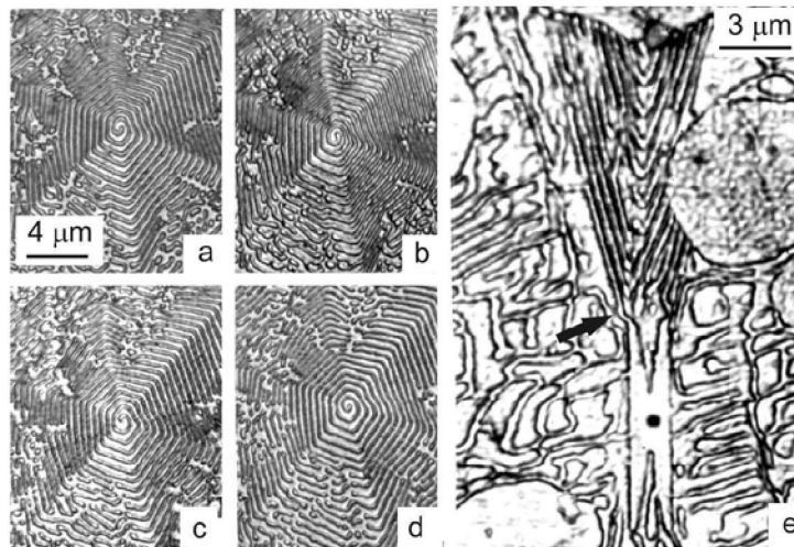
Fig. 16. Spiral conical eutectics \text{Zn} + \text{MgZn}_2 [2]: on the consecutive transversal sections (a-d) the initial spiral turn revolves on its axis; e – longitudinal section through primary prismatic \text{MgZn}_2 crystal. Spiral conical eutectics springs from vertex of the branch of hexagonal prism (arrowed)
