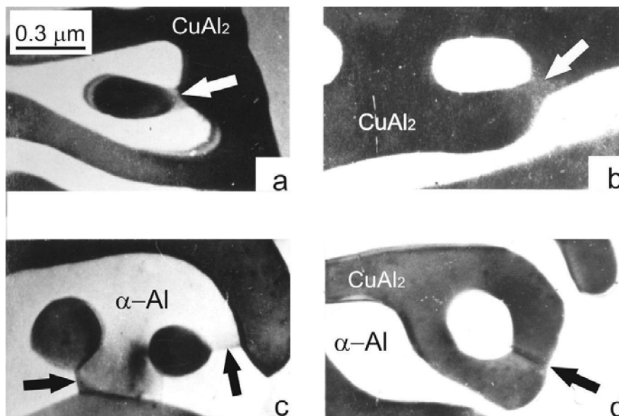
Fig. 19. TEM of thin \text{Al}+\text{CuAl}_2 film without additional thinning: a, b – extremely great rate at which else remains a genetic connection between an elliptic islet and dendrite branch of the given phase (white arrows); c, d – nucleation of the islets of the one phase on the crystallization front of the second one; sub-boundaries (black arrows) show intergrowth of the branches of one phase after environment of the islet of another one
