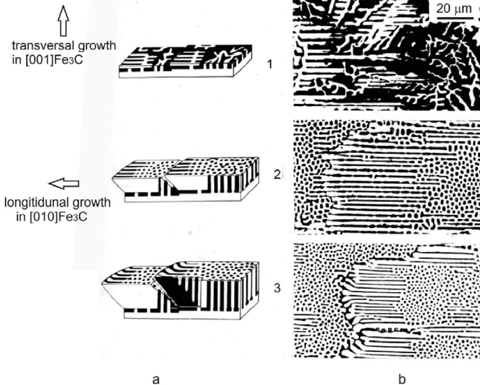
Fig. 7. Stages of eutectic cells formation in ( \gamma\text{-Fe} + \text{Fe}_3\text{C} ) eutectics: \alpha – scheme; \beta – microstructures
