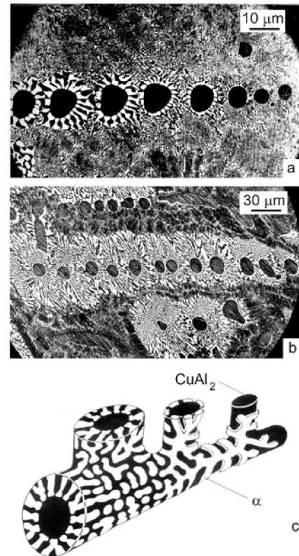
Fig. 14. Growth of eutectics (\text{a-Al}) + \text{CuAl}_2 on a base crystal of the roundish form of growth: a – an initial stage; b – formation cellular boundaries; c – 3D scheme
