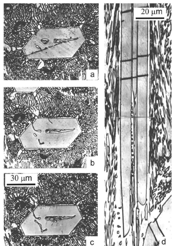
Fig. 15. The morphology of the (\beta\text{-Ti}) + \text{Ti}_3\text{Si}_3 eutectics [2]: a – c – consecutive transversal sections; the basic silicide crystal is in centre of eutectics; d – longitudinal section
