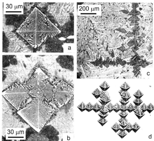
Fig. 13. Dendrite growth of (\gamma\text{-Fe}) + (\text{Mo, Fe})_6\text{C} eutectic colony: a – start of eutectic solidification; b – intermediate stage; c – biphase octahedral dendrite colony; d – 3D scheme
