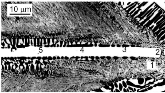
Fig. 5. Transverse cross-section of primary \text{Fe}_3\text{C} crystal showing the initial stages of eutectic grain growth: 1 – quenched liquid phase; 2 – growth of \text{Fe}_3\text{C} crystal with free surface; 3 – growth of \gamma\text{-Fe} dendrite branches (dark); 4 – formation of biphasic ( \gamma\text{-Fe} + \text{Fe}_3\text{C} ) grating; 5 – transversal growth of ( \gamma\text{-Fe} + \text{Fe}_3\text{C} ) eutectics and creation of cellular step on eutectic solidification front
