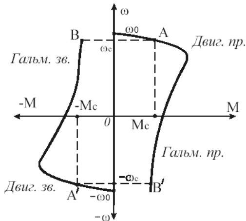
Figure 5.2 – Mechanical characteristics of IM in the drive and breaking modes.
