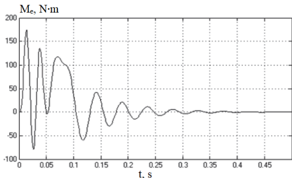
Figure 3. Oscillogram of the electromagnetic torque of the 4A132M4U3 induction motor during a direct start
