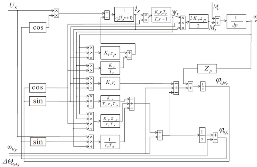
Figure 1. Computational model of an induction motor in i_s - \psi_r variables
