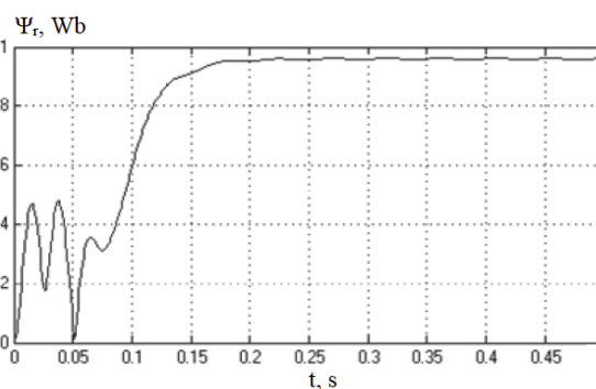
Figure 6. Oscillogram of the change in the rotor winding flux linkage of the 4A132M4U3 induction motor during direct start
